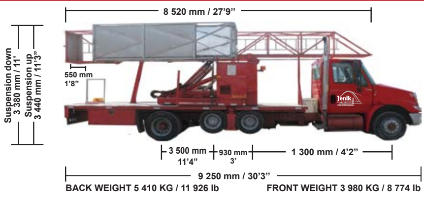
Figure 2 (Tower at lowest level)
