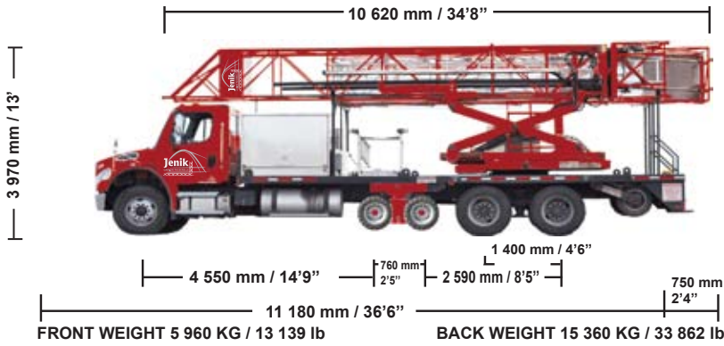
Figure 2 (Tower at lowest level) Open scissor
